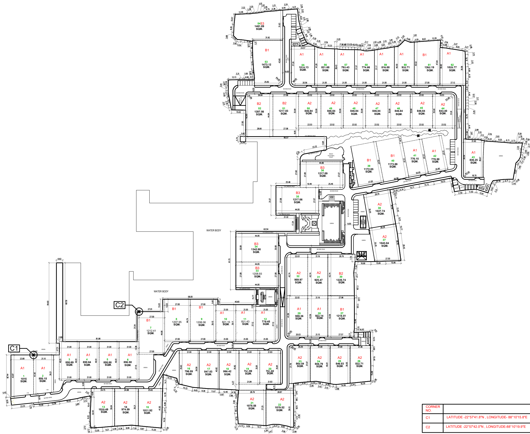
VILLA MASTER PLAN
